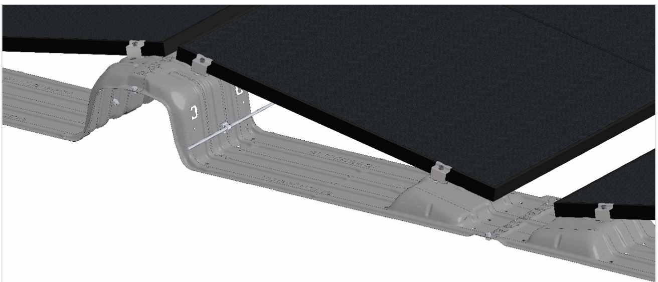
Figure 2: iFIX OW – example showing connection possibilities for equipotential bonding and lightning protection.
